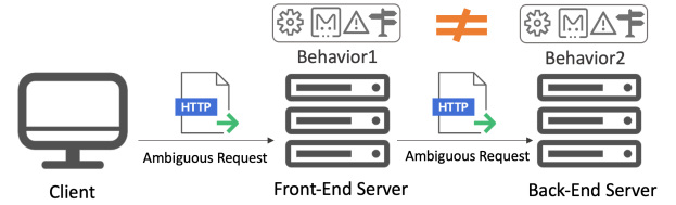
Fig. 2: Semantic Gap Attack: different behavior when parsing an ambiguous HTTP message.
